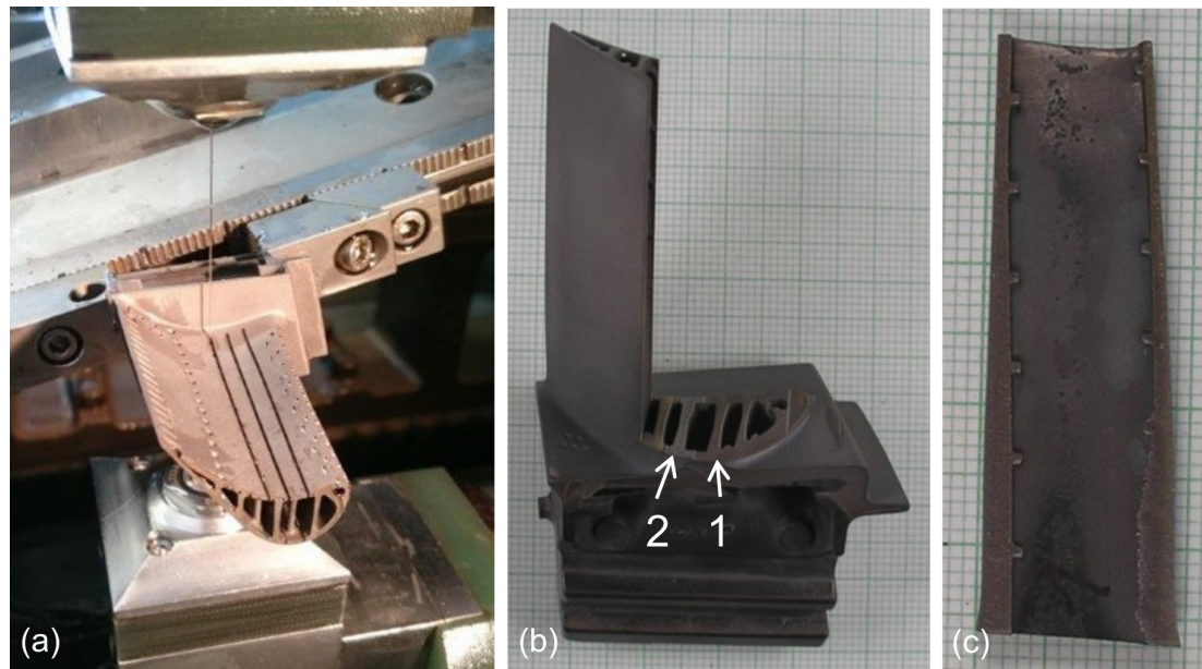
Figure 2. Sample extraction from cooling channel partition walls from a high pressure turbine blade. (a) Cutting by wire electro discharge erosion, (b) location of partition walls suitable for specimen manufacturing, and (c) sample from position 1 in (b).
