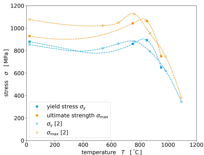
Figure 5. Comparison of temperature dependent yield stress and tensile strength values with literature values from [2].
