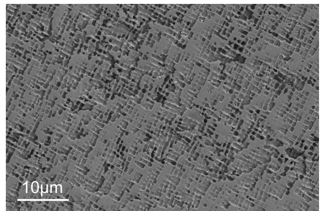
Figure 3. Micrograph by scanning electron microscopy from a polished and etched surface of a cooling channel partition wall extracted from a used turbine blade. Material is René N5, and the micrograph displays the typical microstructure with cubic \gamma' precipitates aligned along crystallographic \langle 100 \rangle directions.
