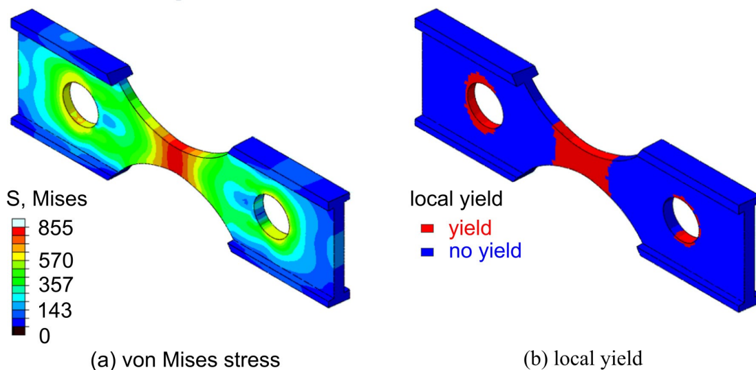
Figure 4. Stress distribution (a) and local yield (b), calculated by finite element simulation for the final specimen geometry under tensile load applied at the bolt holes (von Mises equivalent stresses in MPa).
