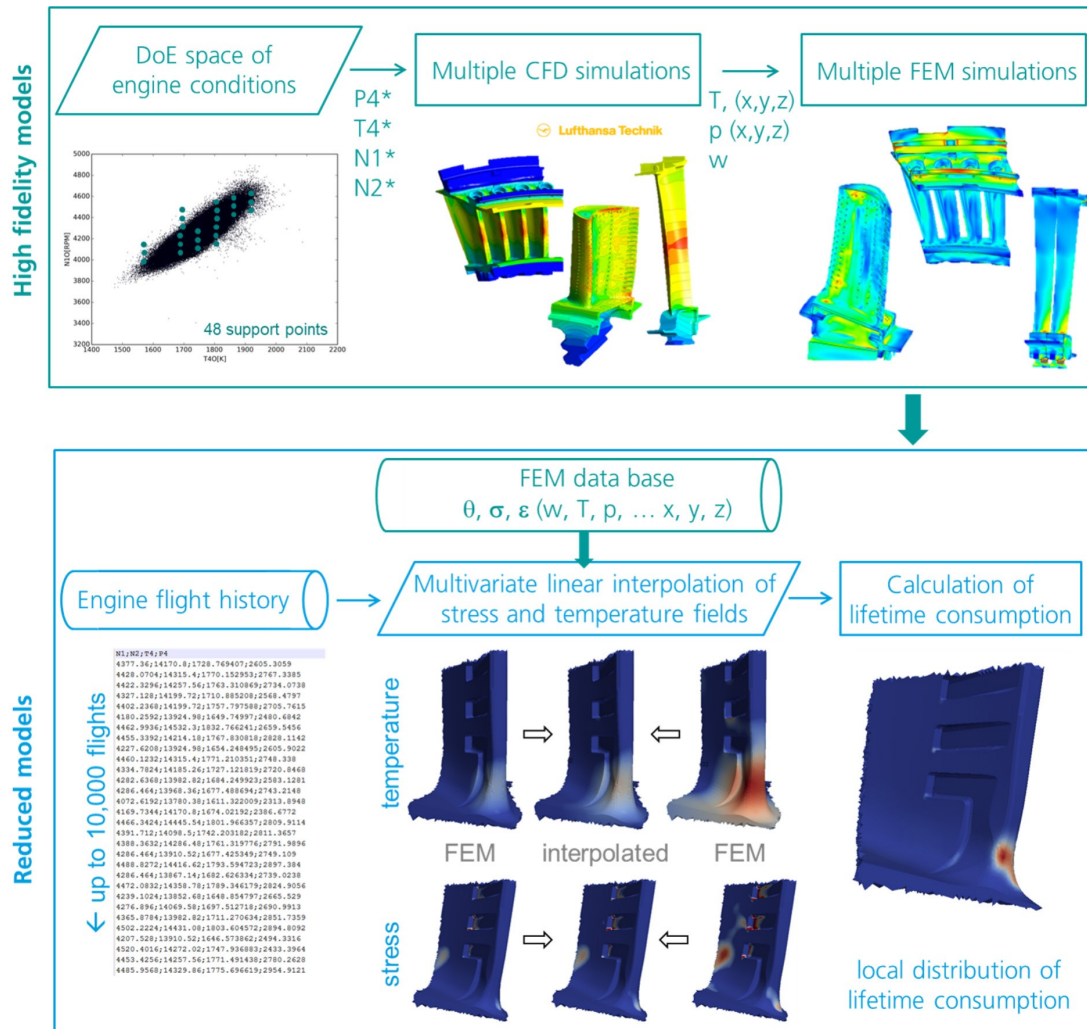
Figure 1. Schematic process of lifetime post processor in accordance with [1].
