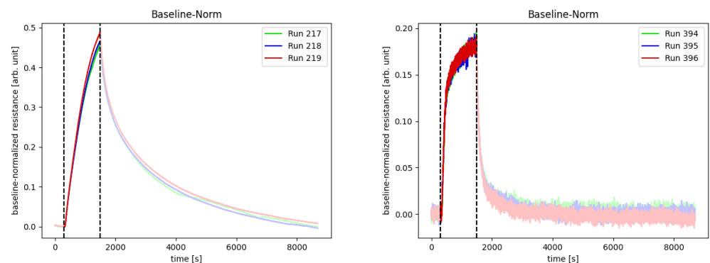
Figure 8. Midfield place of worst sensor in the ranking.
