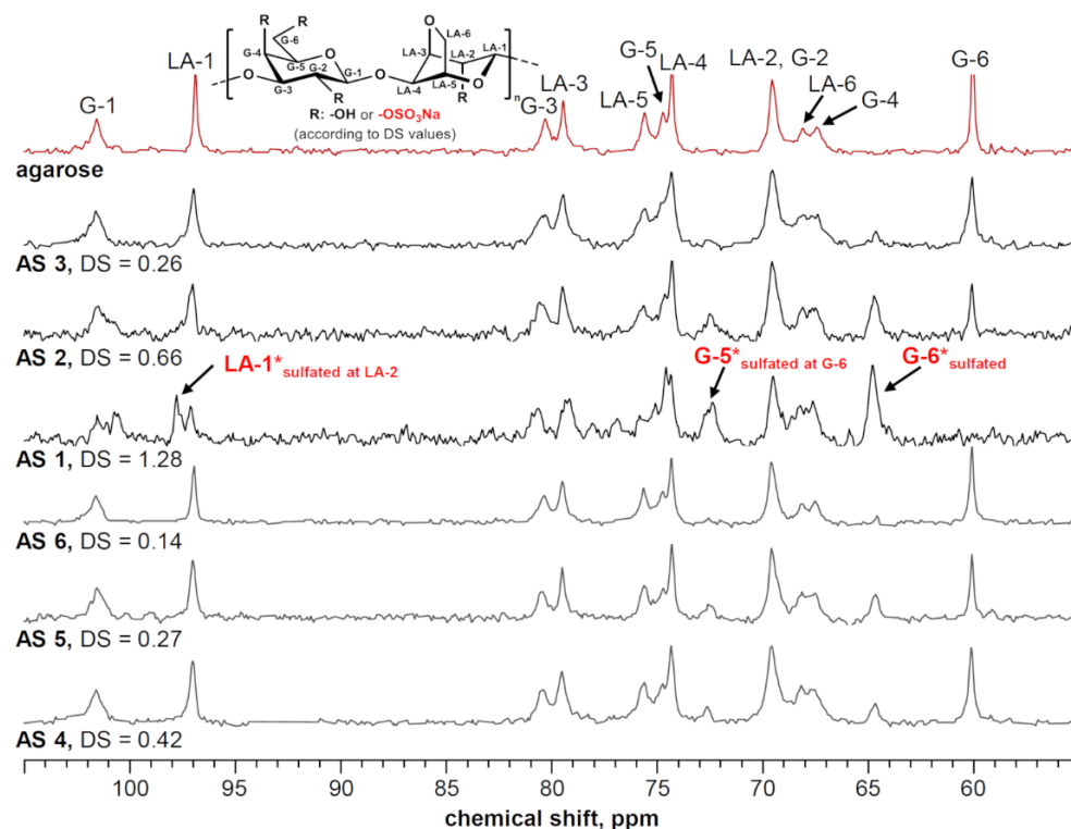
Figure 2. 13 C NMR spectra (recorded in DMSO-d 6 ) of agarose and agarose sulfates (AS) with different degrees of substitution (DS) that were prepared by homogeneous synthesis in different reaction media. Positions that were directly affected by a functionalization with sulfate groups were marked (*).
