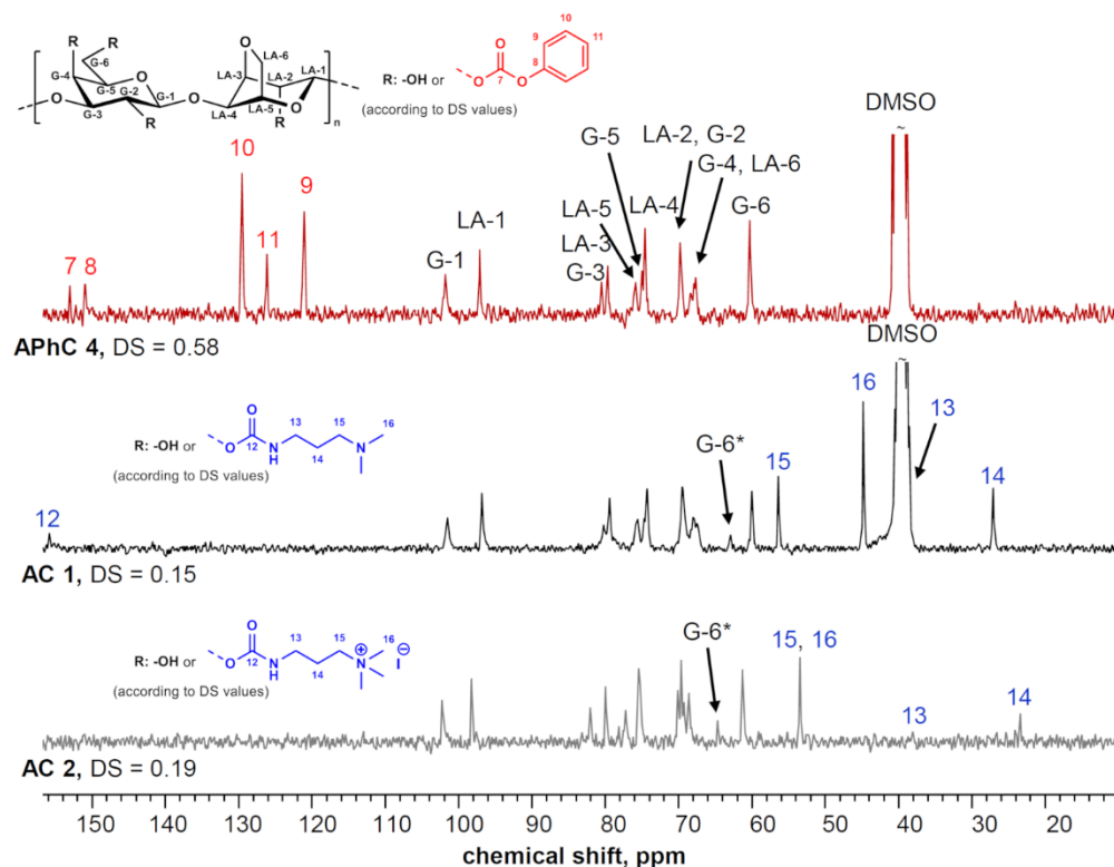
Figure 3. ^{13}\text{C} NMR spectra (recorded in \text{DMSO-d}_6 or \text{D}_2\text{O} at 60^\circ\text{C} ) of agarose phenyl carbonate (APhC) and agarose carbamates (ACs) with different degrees of substitution (DS). Positions that were directly affected by a functionalization with carbamate groups were marked (*).
