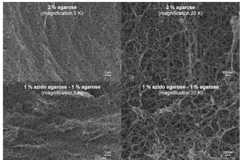
Figure 5. Scanning electron microscopy images of hydrogels obtained from agarose or agarose together with azido agarose after critical point drying.
