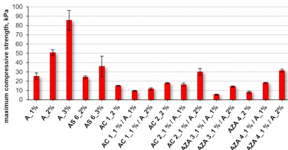
Figure 4. Results of mechanical tests obtained for different hydrogels derived from agarose (A), agarose sulfates (ASs), azido agarose (AZA), agarose carbamates (ACs), or mixtures therefrom.
