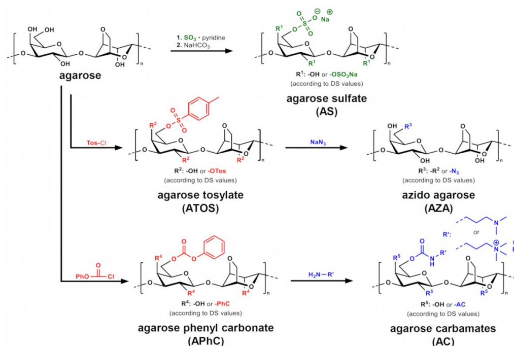
Figure 1. Reaction scheme for the synthesis of the different agarose derivatives prepared in this study.
