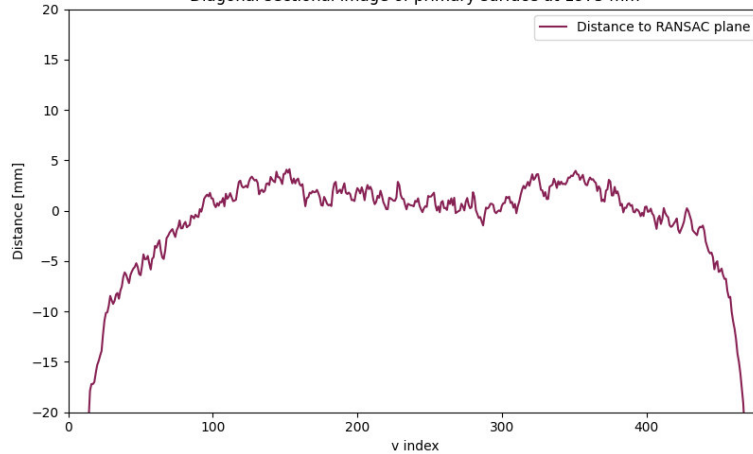
Diagonal sectional image of primary surface at 1975 mm
