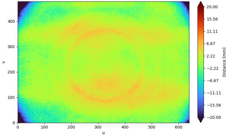
Distances to middle (RANSAC) plane at 1975 mm
