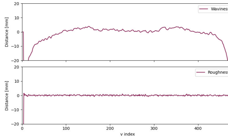
Diagonal sectional image of waviness and roughness surface at 1975 mm
